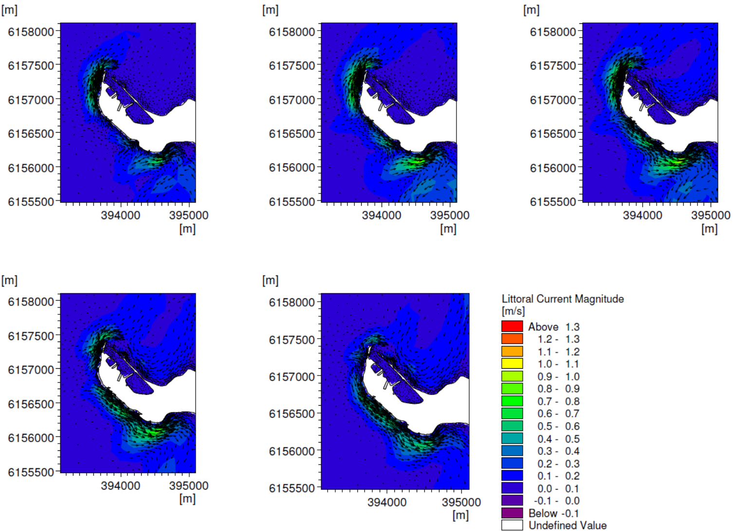
Figure 6.3 Littoral current magnitude and directions at Troon for force 8 gales between directions 180°N to 300°N with sea level rise applied
