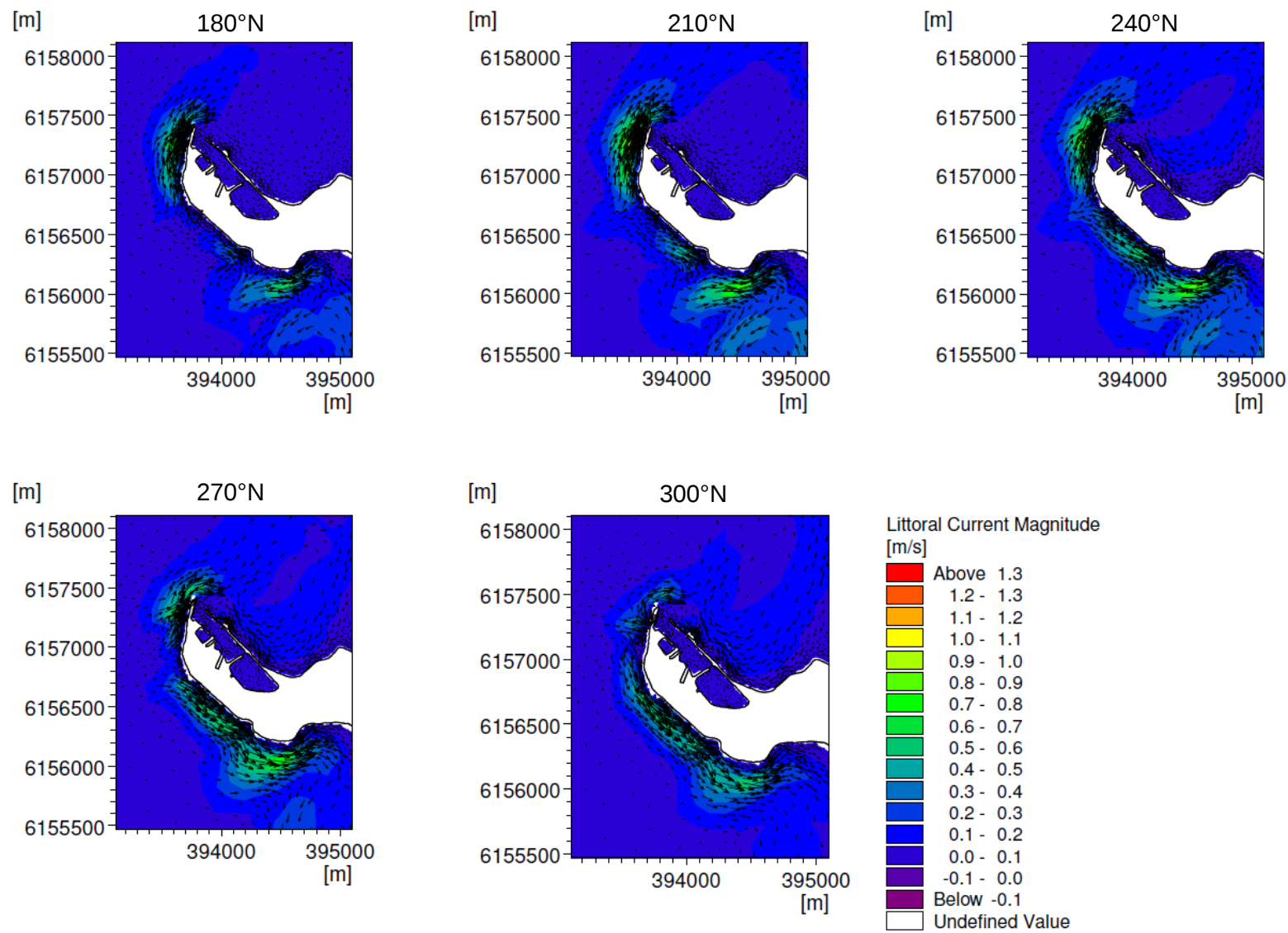
Figure 4.7 Littoral current magnitude and directions at Troon for force 8 gales between directions 180°N to 300°N
